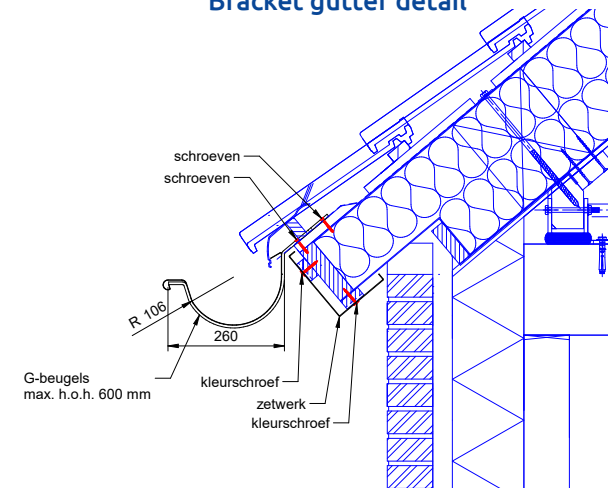
Bracket gutter detail
