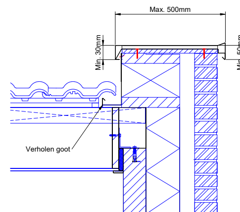
Capping detail
